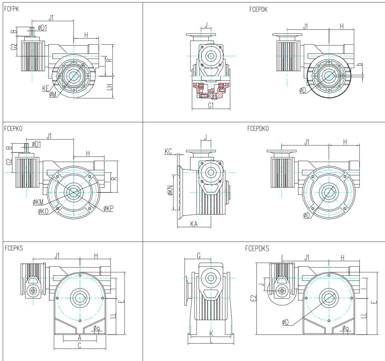
Double Stage FCEP (Worm-Worm) Series Mounting Dimension Data Table:
