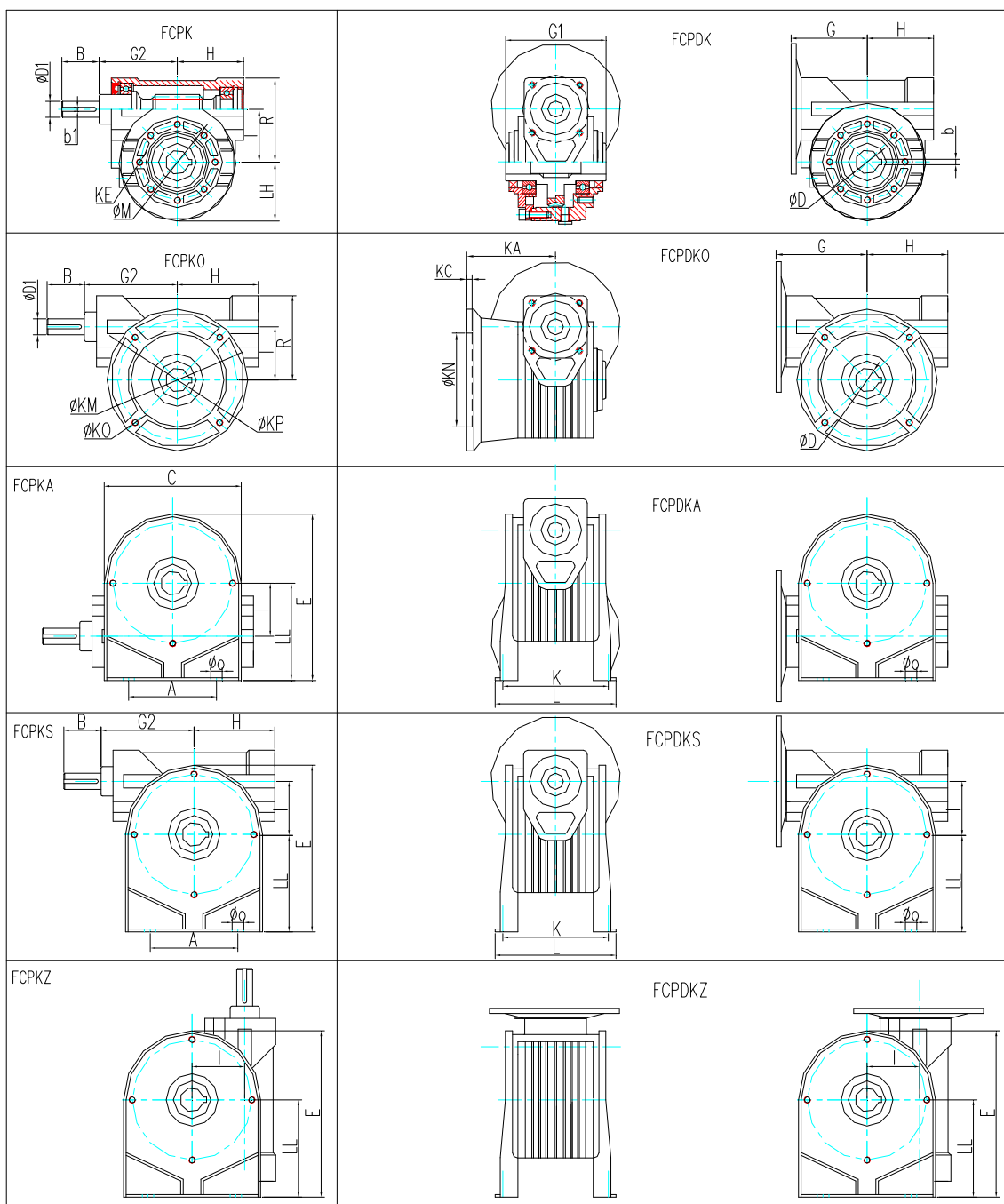
Single Stage FCP Series Mounting Dimension Data Table
